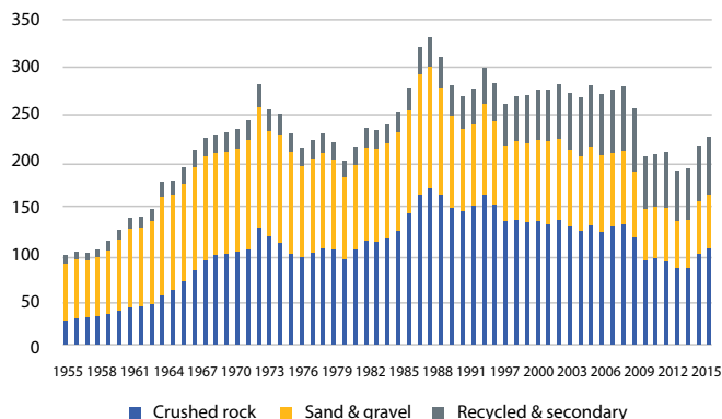
Chart 6. Aggregates sales by sources of supply (GB)
